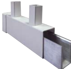
Commercial Reinforced Top and Bottom Rail
